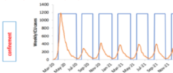
Figure 4: Illustration of adaptive triggering of suppression strategies in GB, for R_t < 2.2 , a policy of all four
