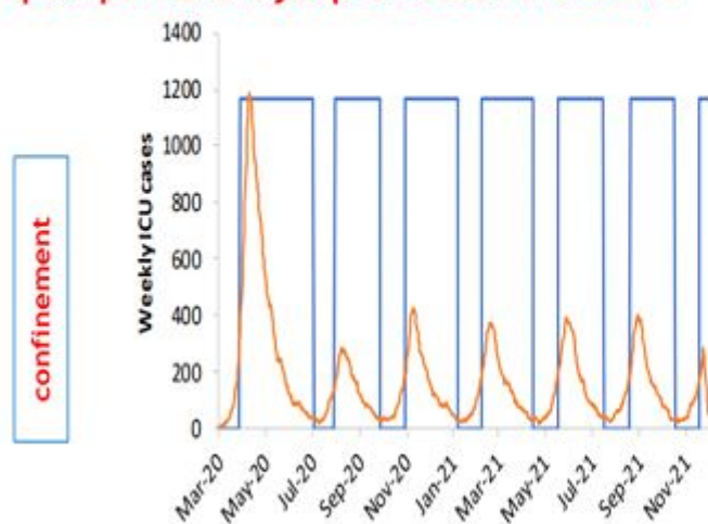
Figure 4: Illustration of adaptive triggering of suppression strategies in GB, for R_0=2.2 , a policy of all four
