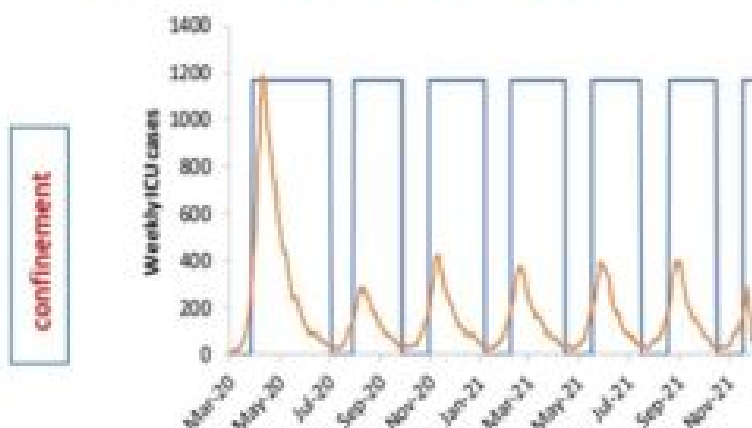
Figure 4: Illustration of adaptive triggering of suppression strategies in GB, for R=2.2 , a policy of all flow
